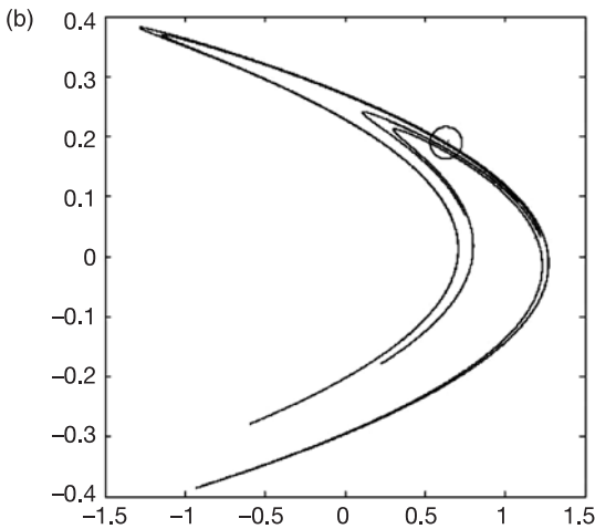
16. Two-dimensional plots of (a) a slice of the Moore-Spiegel attractor at z=0 ; and (b) the Hénon attractor where \alpha is 1.4 and \beta is 0.3. Note the similar structure with many leaves in each case
