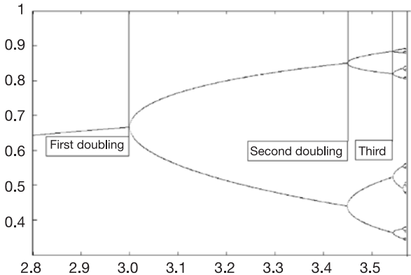
11. Period doubling behaviour in the Logistic Map as a increases from 2.8 to \sim 3.5 ; the first three doublings are marked
